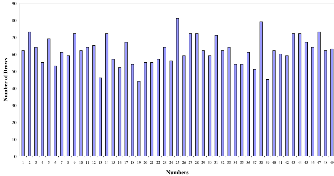
Chart 2 - Frequency of Lottery Numbers - in numerical order (out of possible 434)
