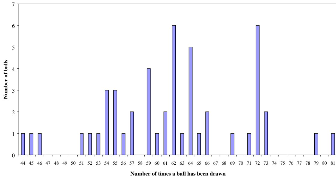
Chart 3 - Frequency Distribution of Lottery Balls
