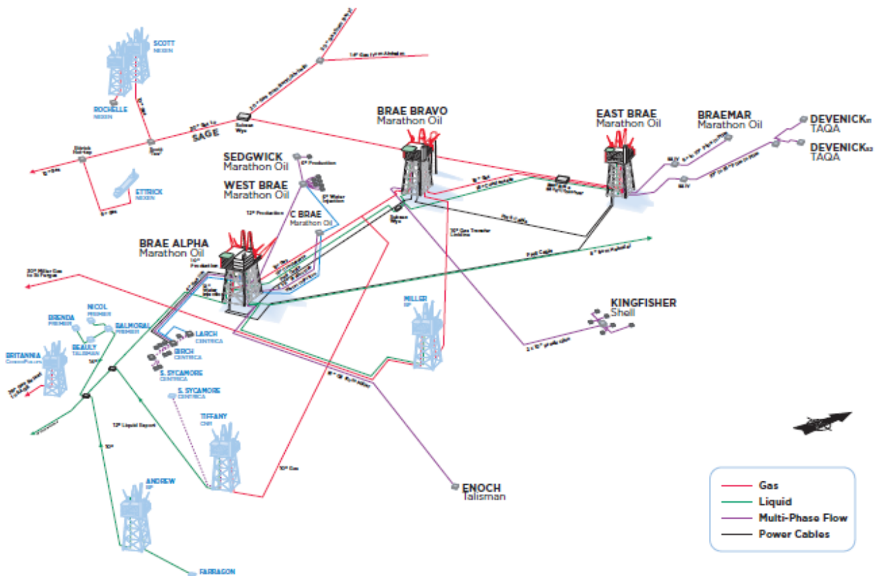
“Brae Area Schematic demonstrates the operational and commercial complexity of the UKCS...”
